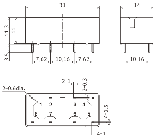
External dimensions
