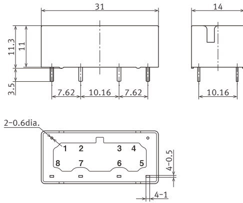
External dimensions
