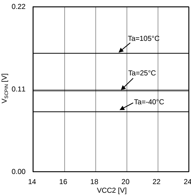
Figure 54. SCPIN Input voltage vs. VCC2 (ISCPIN=1mA)
