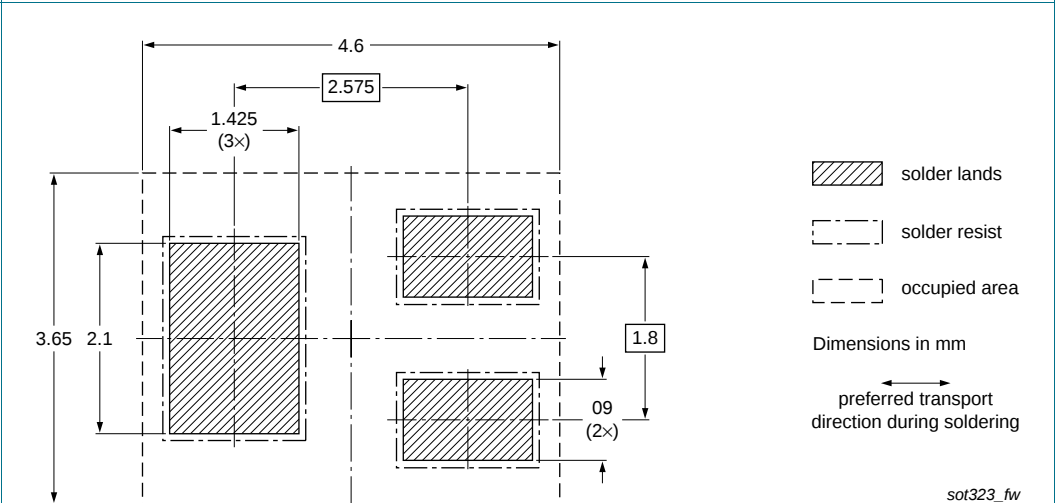
Fig 21. Wave soldering footprint PDTA124EU (SOT323/SC-70)
