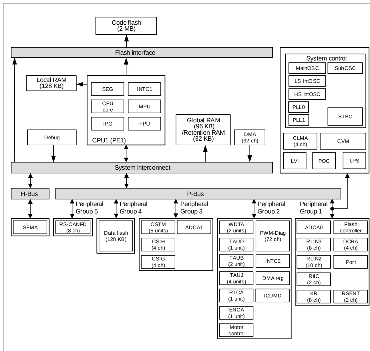
Figure 1B.8 Internal Block Diagram (RH850/F1KM-S2 176-Pin Version)
