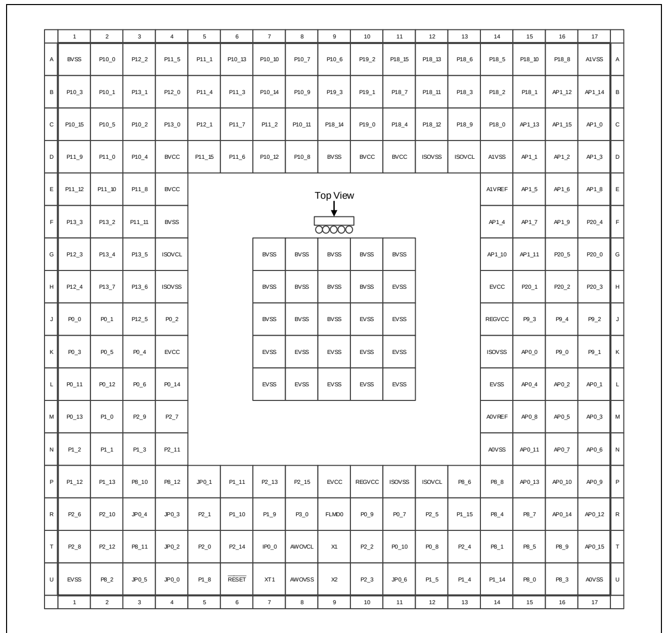
Figure 2B.4 Pin Connection Diagram in RH850/F1KM-S4 (233-Pin FCBGA)
