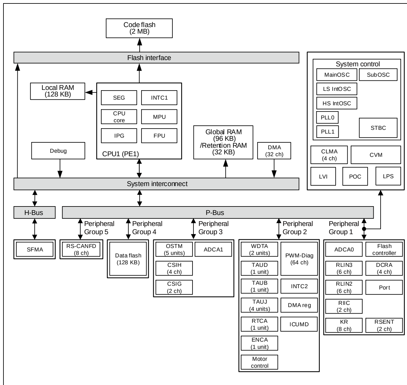
Figure 1B.7 Internal Block Diagram (RH850/F1KM-S2 144-Pin Version)
