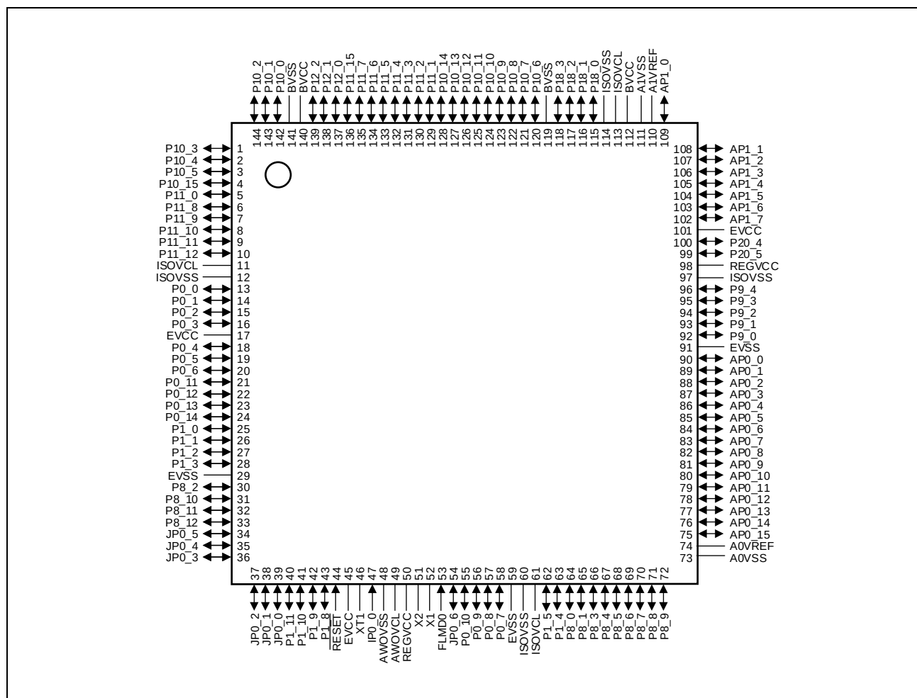
Figure 2B.2 Pin Connection Diagram in RH850/F1KM-S4 and RH850/F1KM-S2 (144-Pin LQFP)
