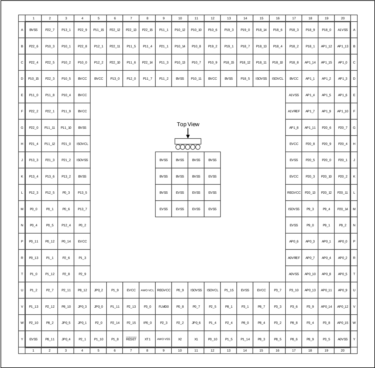
Figure 2B.5 Pin Connection Diagram in RH850/F1KM-S4 (272-Pin FPBGA)
