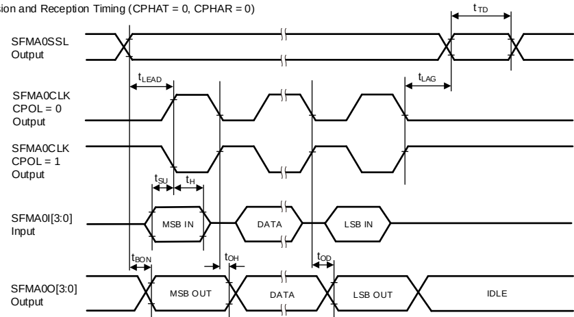
Transmission and Reception Timing (CPHAT = 0, CPHAR = 0)
