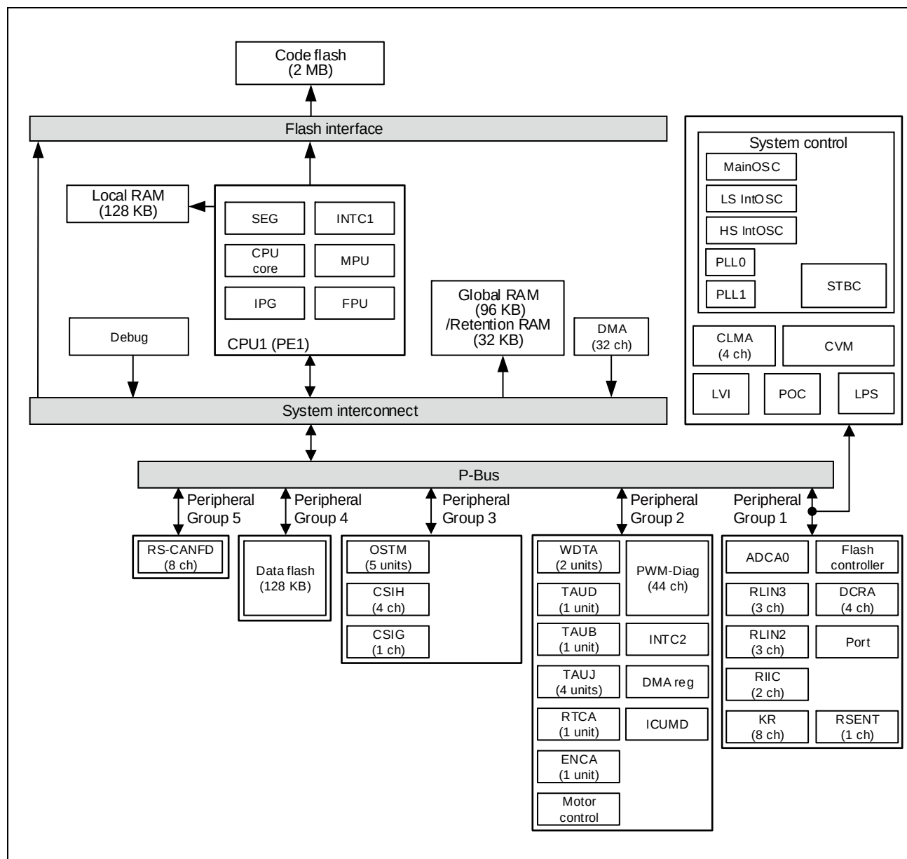
Figure 1B.6 Internal Block Diagram (RH850/F1KM-S2 100-Pin Version)
