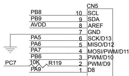
Figure 2. X-NUCLEO-BNRG2A1 schematic diagram - Arduino connectors
