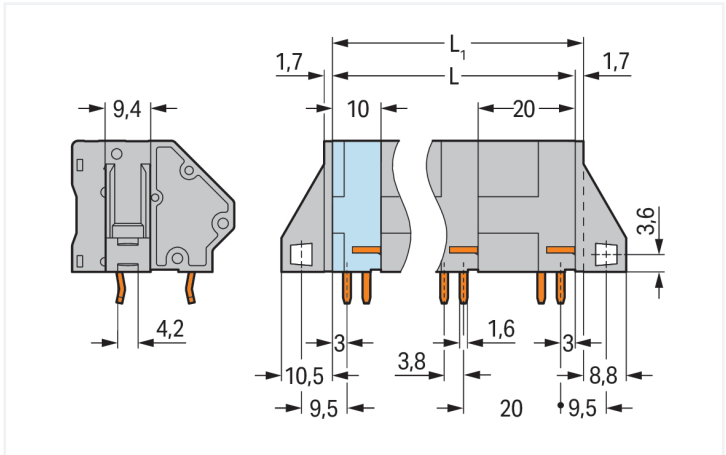
Dimensions in mm L = (pole no. – 1) x pin spacing + 10 mm L1 = L + 1.7 mm ± version without mounting flange
