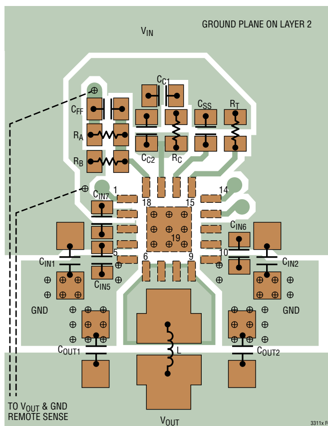
Figure 4. Recommended PCB Layout for the LTC3311
