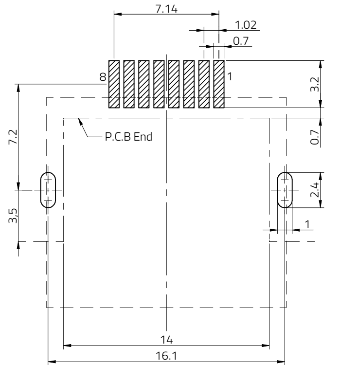
General tolerance: 0.05mm Scale-4:1
