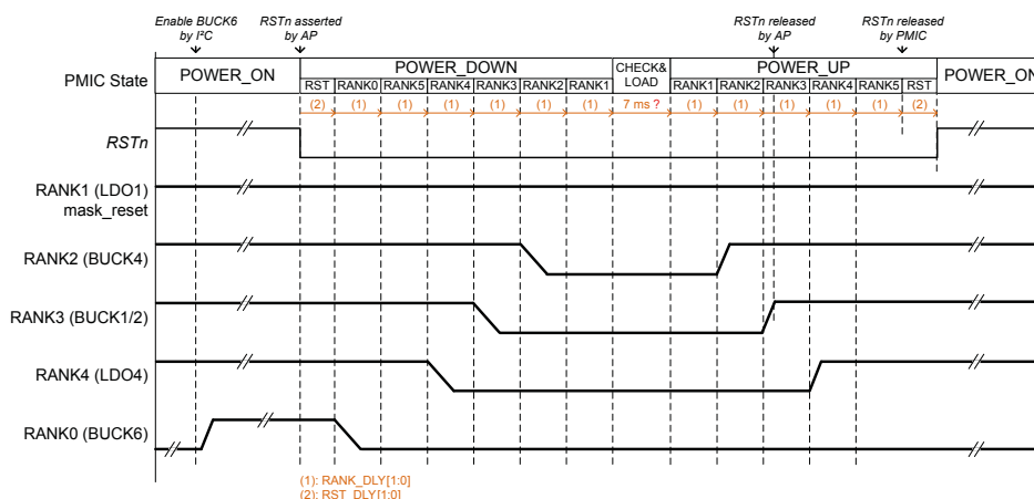
Figure 18. Reset power-cycle sequence example
