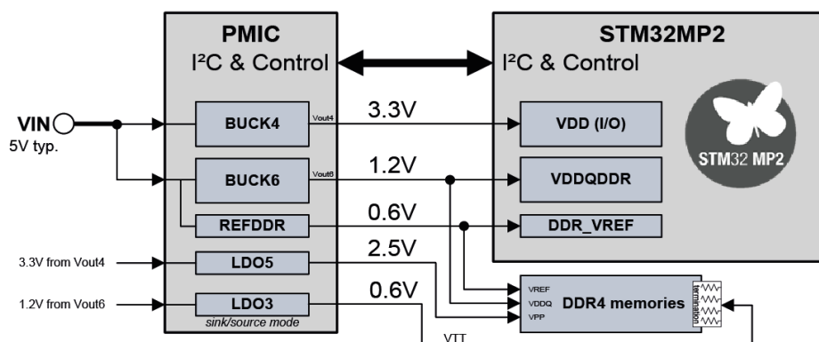
Figure 5. LDO3 uses in sink/source mode with DDR4
