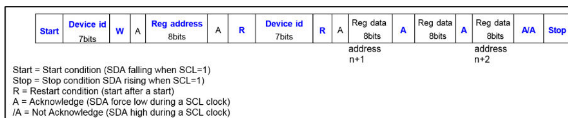
Figure 20. I 2 C read operation
