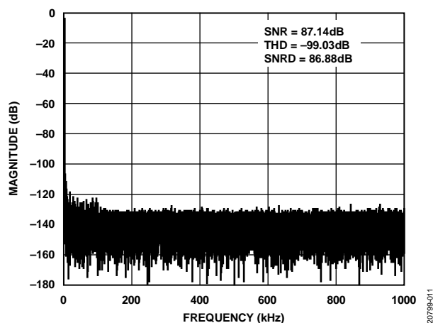
Figure 9. FFT, V_{REF} = 3.3 V External
