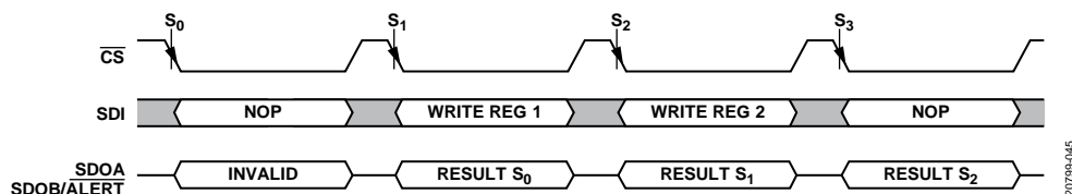
Figure 43. Register Write
