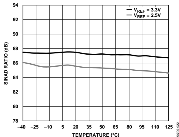
Figure 20. SINAD Ratio vs. Temperature
