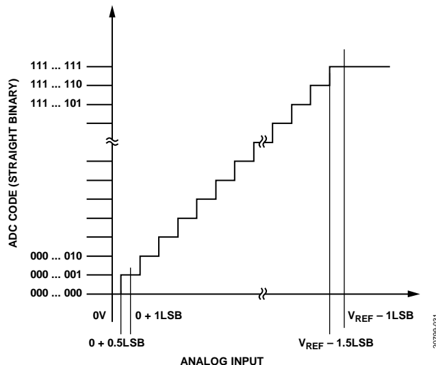
Figure 29. ADC Ideal Transfer Function (FSR = Full-Scale Range)
