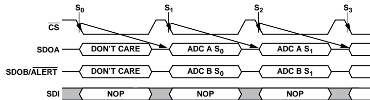
Figure 39. Reading Conversion Results for 2-Wire Mode
