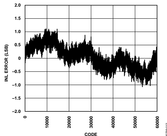
Figure 11. Integral Nonlinearity (INL) Error
