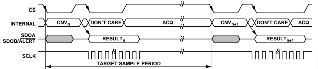
Figure 41. Low Throughput Low Latency
