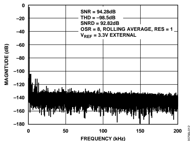
Figure 10. FFT with Oversampling
