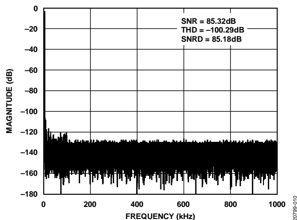
Figure 8. Fast Fourier Transform (FFT), V_{REF} = 2.5 V Internal
