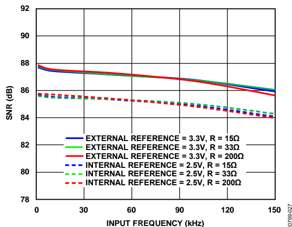
Figure 25. SNR vs. Input Frequency
