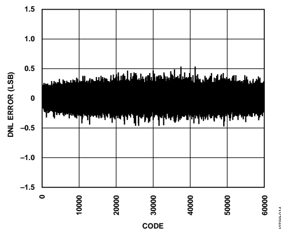
Figure 12. Differential Nonlinearity (DNL) Error
