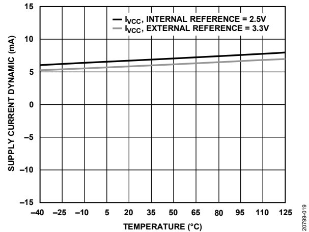
Figure 17. Supply Current Dynamic vs. Temperature
