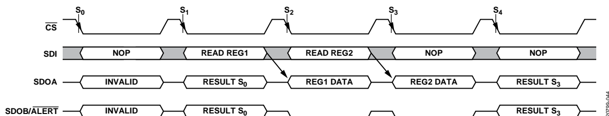
Figure 42. Register Read
