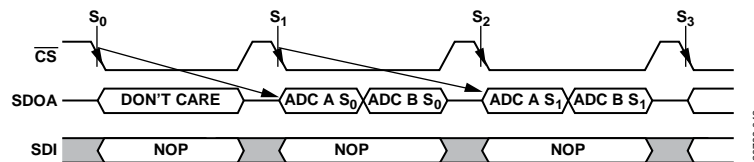
Figure 40. Read Conversion Results for 1-Wire Mode
