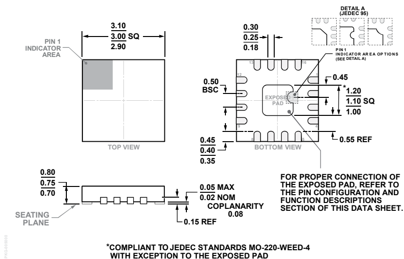
Figure 45. 16-Lead Lead Frame Chip Scale Package [LFCSP] 3 mm × 3 mm Body and 0.75 mm Package Height (CP-16-45)
