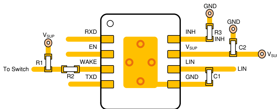
Figure 10-4. Layout Example
