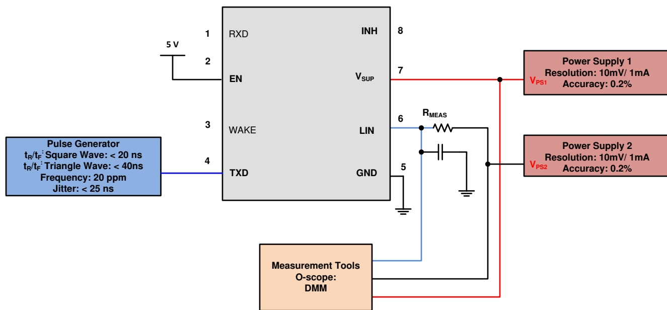
Figure 8-10. Test Circuit for I_{BUS\_NO\_BAT} Loss of Battery
