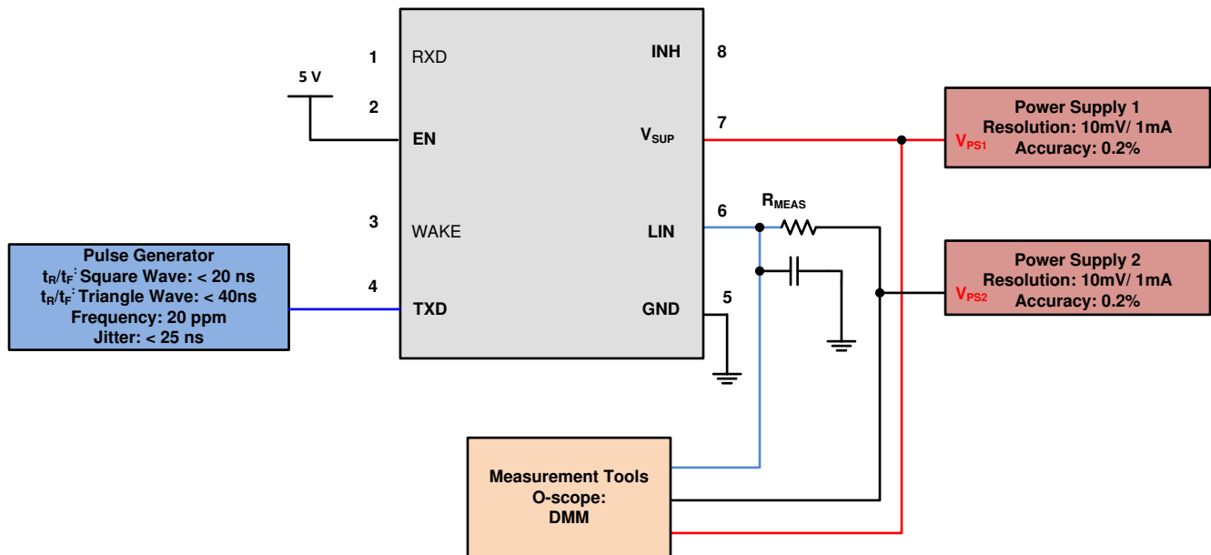
Figure 8-13. Propagation Delay Test Circuit; Param 31, 32
