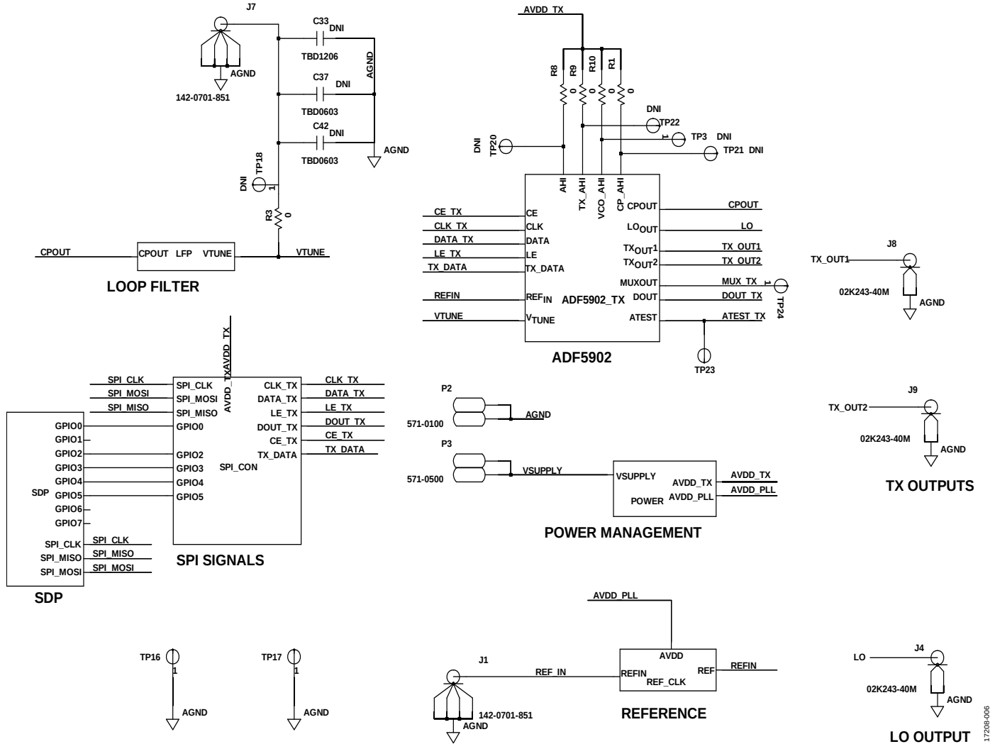
Figure 6. EV-ADF5902SD1Z Evaluation Board Schematic (Page 1)
