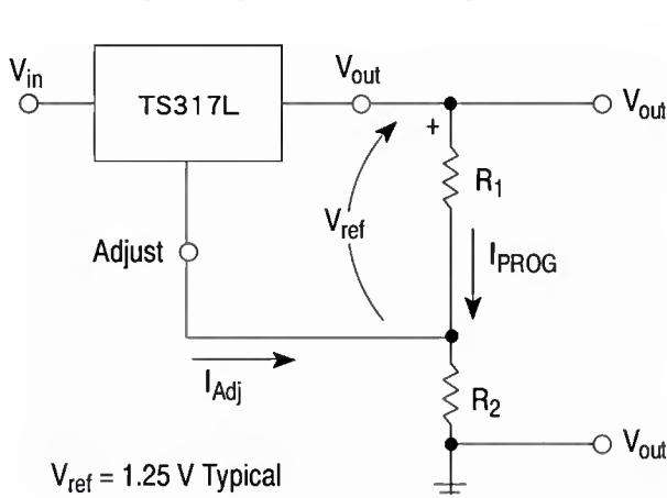
Figure 17. Basic Circuit Configuration
