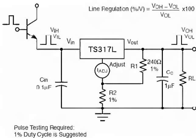
Figure 3. Standard Test Circuit
