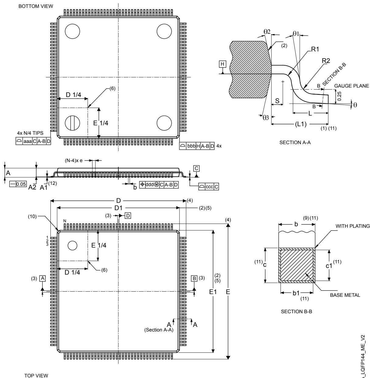
Figure 58. LQFP144 - Outline (15)
