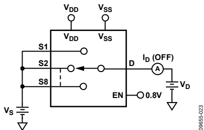
Figure 20. I_D (Off)
