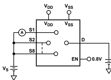
Figure 22. Input Leakage Current (with Overvoltage)
