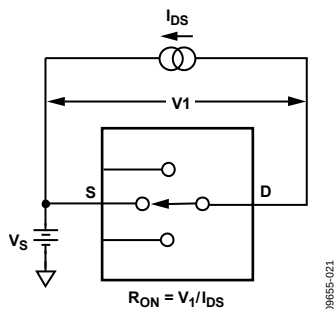
Figure 18. On Resistance
