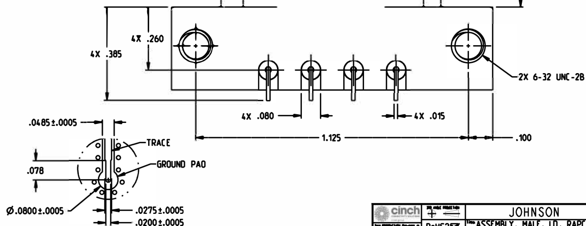
MOUNTING FOOTPRINT (EACH PORT, TOP VIEW)
