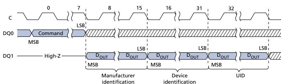
Figure 10: READ ID and MULTIPLE I/O READ ID Commands
