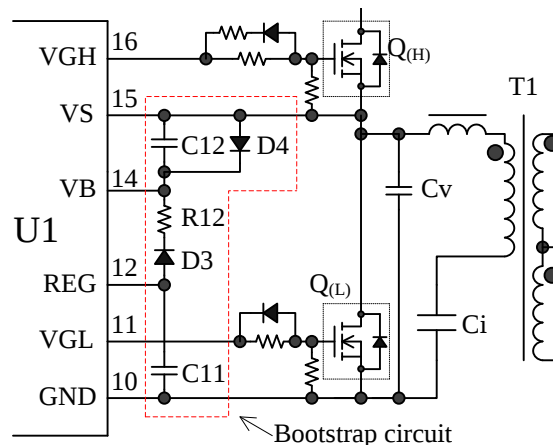
Figure 8-17. Bootstrap circuit
