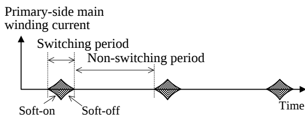
Figure 8-19. Standby waveform
