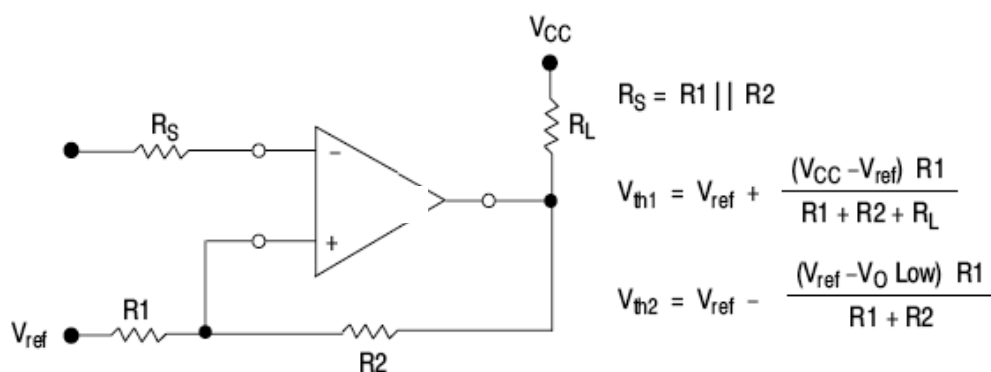
Figure 8. Comparator with Hysteresis
