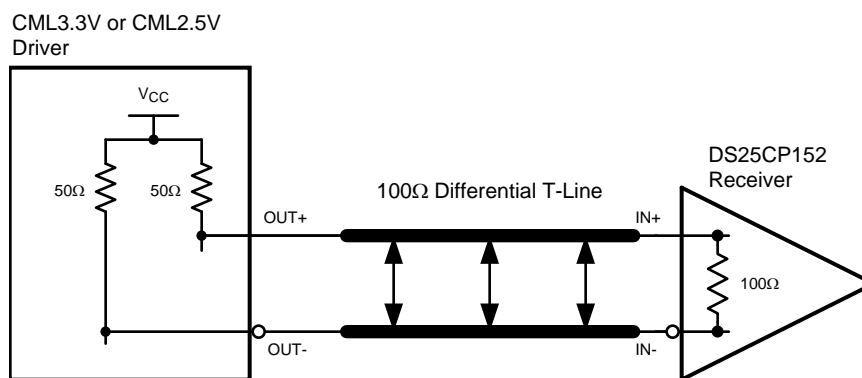
Figure 3. Typical CML Driver DC-Coupled Interface to DS25CP152Q Input
