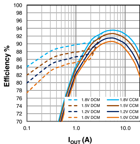
Figure 19: Efficiency, V_{\text{IN}}=5\text{V}
