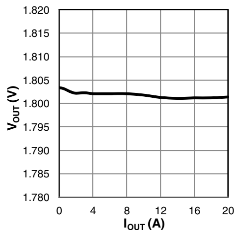
Figure 1: Load Regulation
