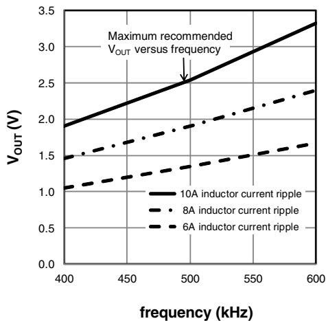
Figure 12: V_{OUT} versus f , V_{IN}=12V
