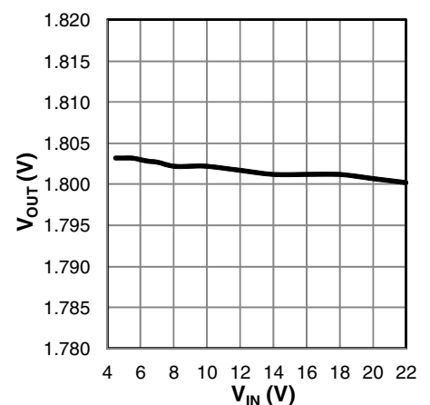
Line Regulation
