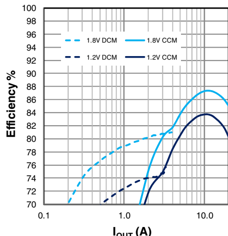
Figure 23: Efficiency, V_{\text{IN}}=19.6\text{V}
