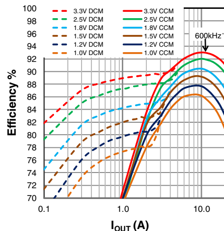
Figure 21: Efficiency, V_{\text{IN}}=12\text{V}
