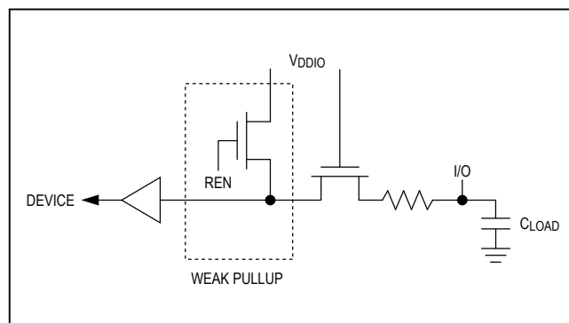
Figure 1. GPIO
