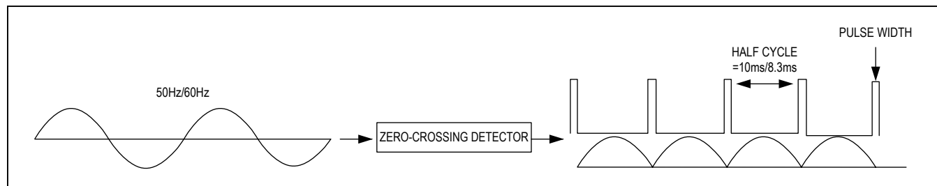
Figure 4. Zero-Crossing AC Detector
