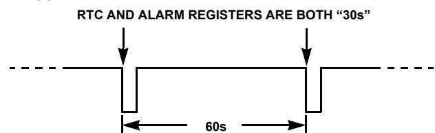
FIGURE 14. \overline{\text{IRQ}}/\text{F}_{\text{OUT}} WAVEFORM
