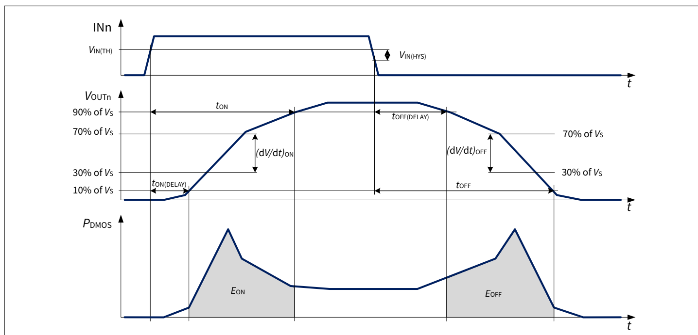
Figure 17 Switching a resistive load
