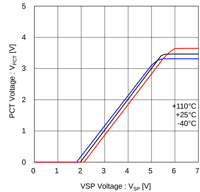
Figure 27. VSP vs PCT Offset Voltage
