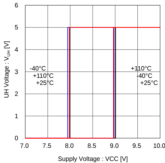
Figure 26. Under Voltage Lock Out (VCC)
