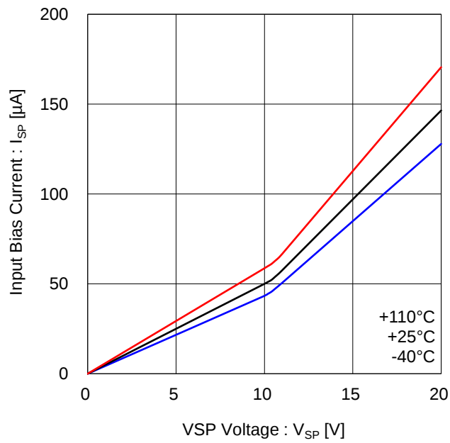
Figure 14. VSP Input Bias Current
