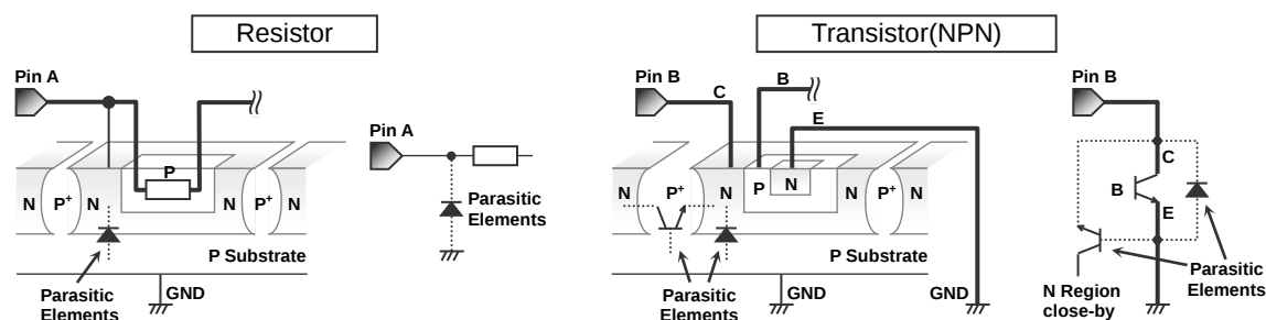
Figure 42. Example of Monolithic IC structure
