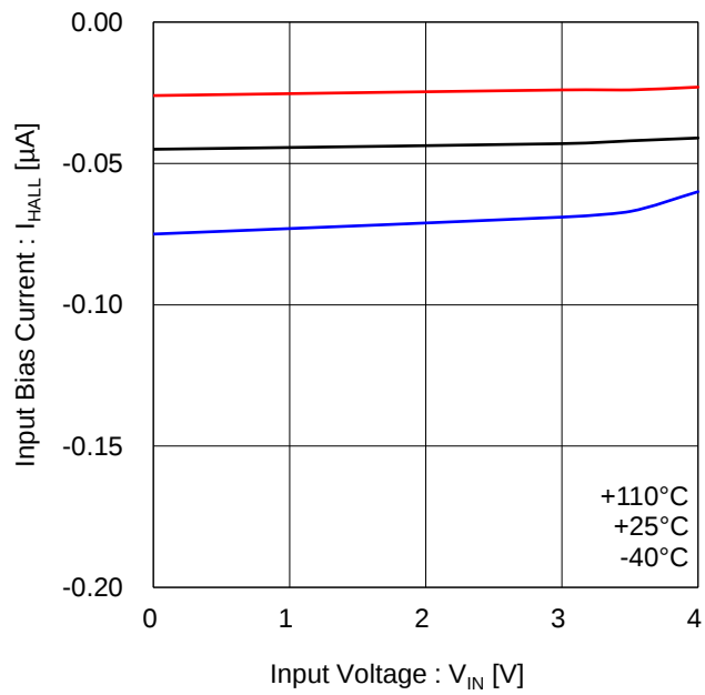
Figure 12. Hall Comparator Input Bias Current (HXP, HXN)
