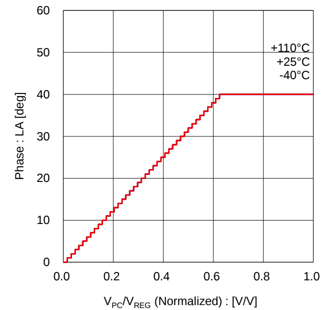
Figure 29. PC Voltage Normalized vs Lead Angle
