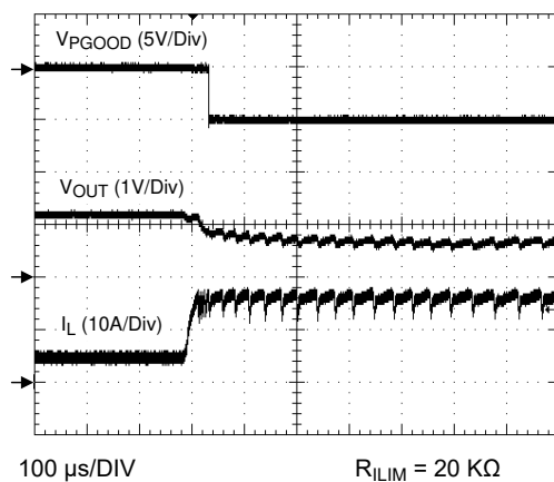
Figure 6-19. Output Overcurrent Condition
