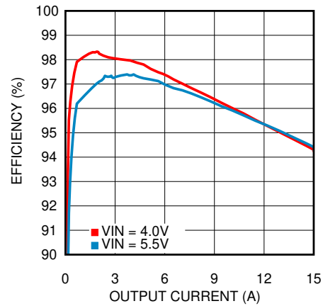
Figure 6-2. Efficiency
