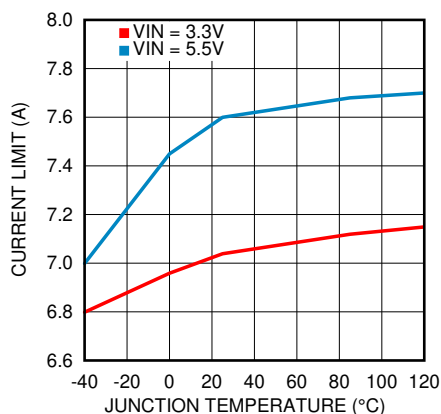
Figure 6-15. Peak Current Limit ( I_{CLR} ) vs Temperature
