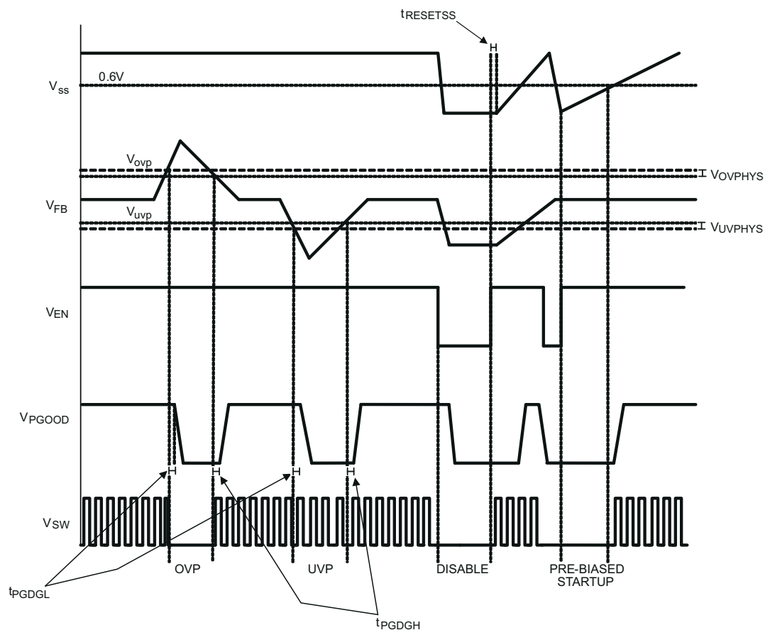
Figure 7-2. PGGOOD Conditions
