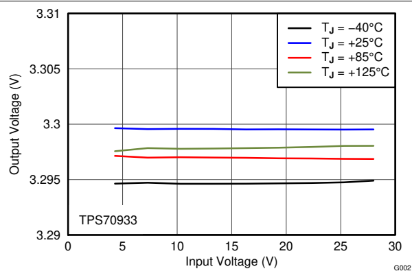
Figure 6-2. 3.3-V Line Regulation vs V_{\text{IN}} and Temperature
