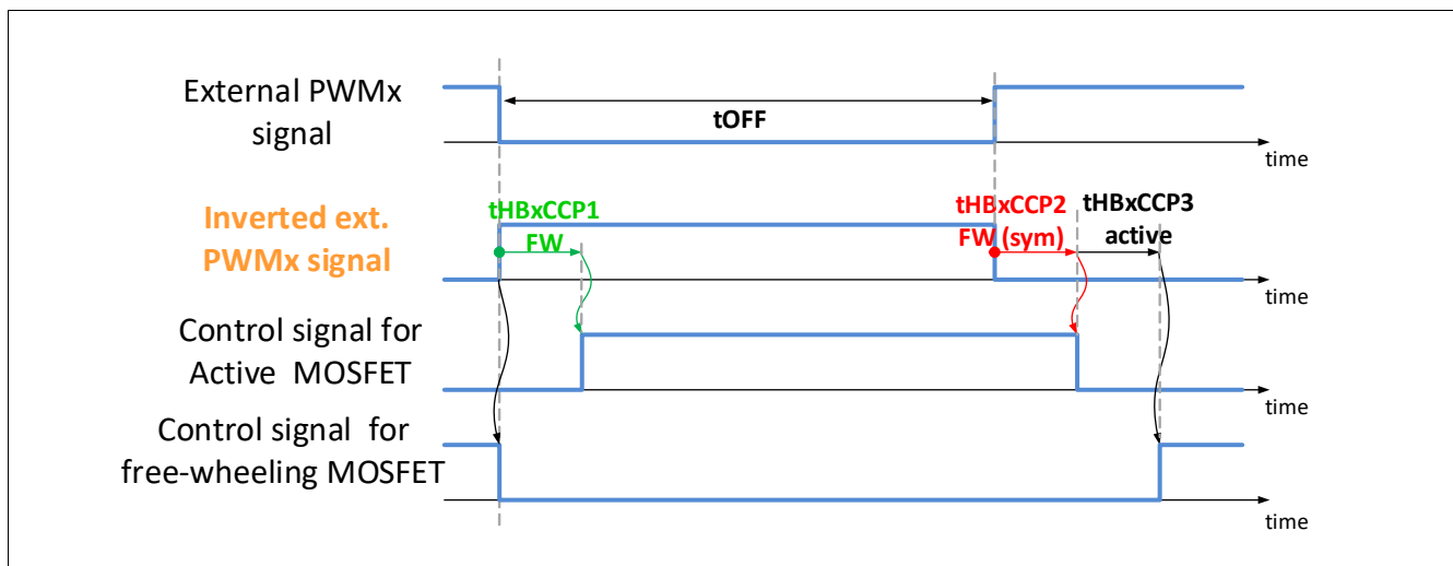
Figure 28 Internal signals for PWM operation - General case: t_{OFF} > t_{HBxCCP\text{ FW}} , t_{ON} > t_{HBxCCP\text{ active}} , motor operating as generator
