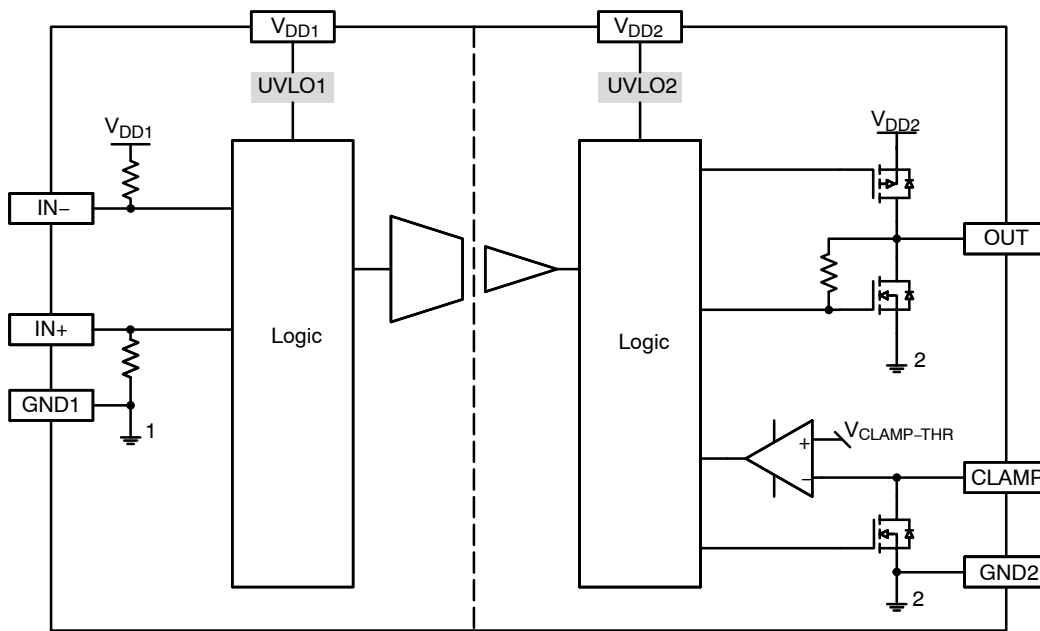
Figure 2. Simplified Block Diagram, NCx5708zA
