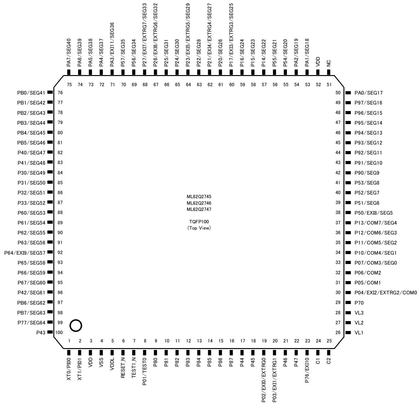
Fig.3-1 100 pin TQFP
