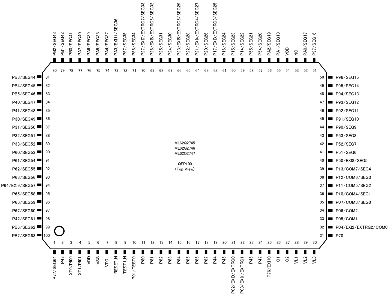
Fig.3-2 100 pin QFP
