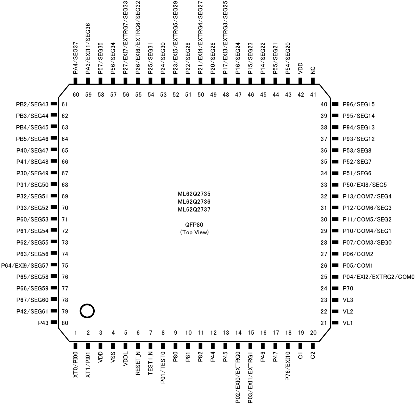
Fig.3-3 80 pin QFP
