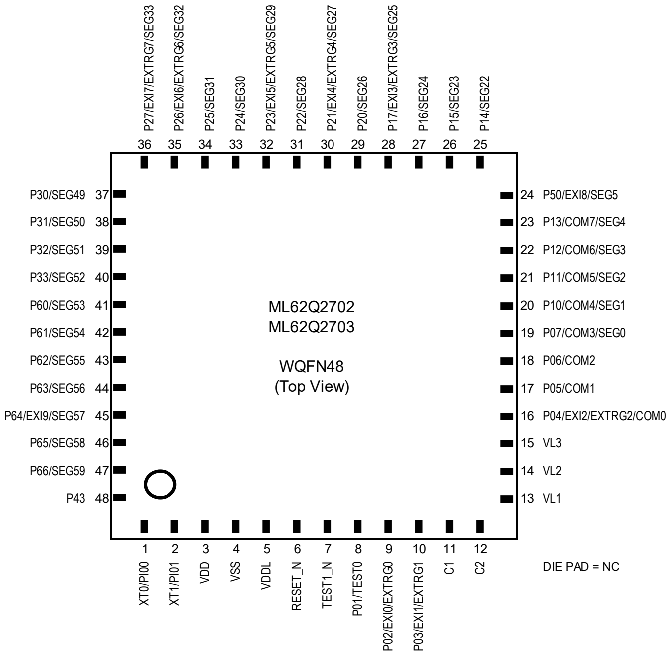
Fig.3-6 48 pin WQFN
