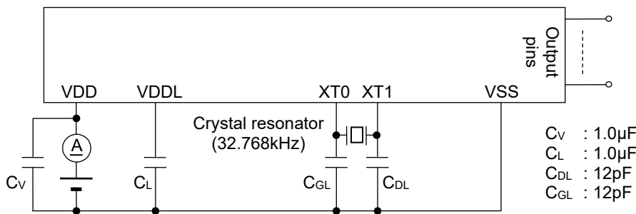
Measuring circuit 2
