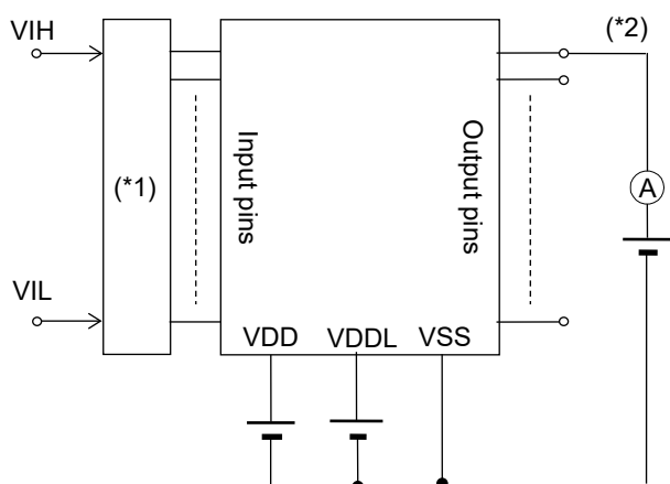
Measuring circuit 5
