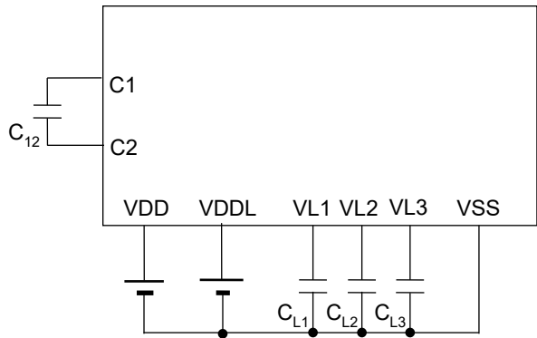
Measuring circuit 6
