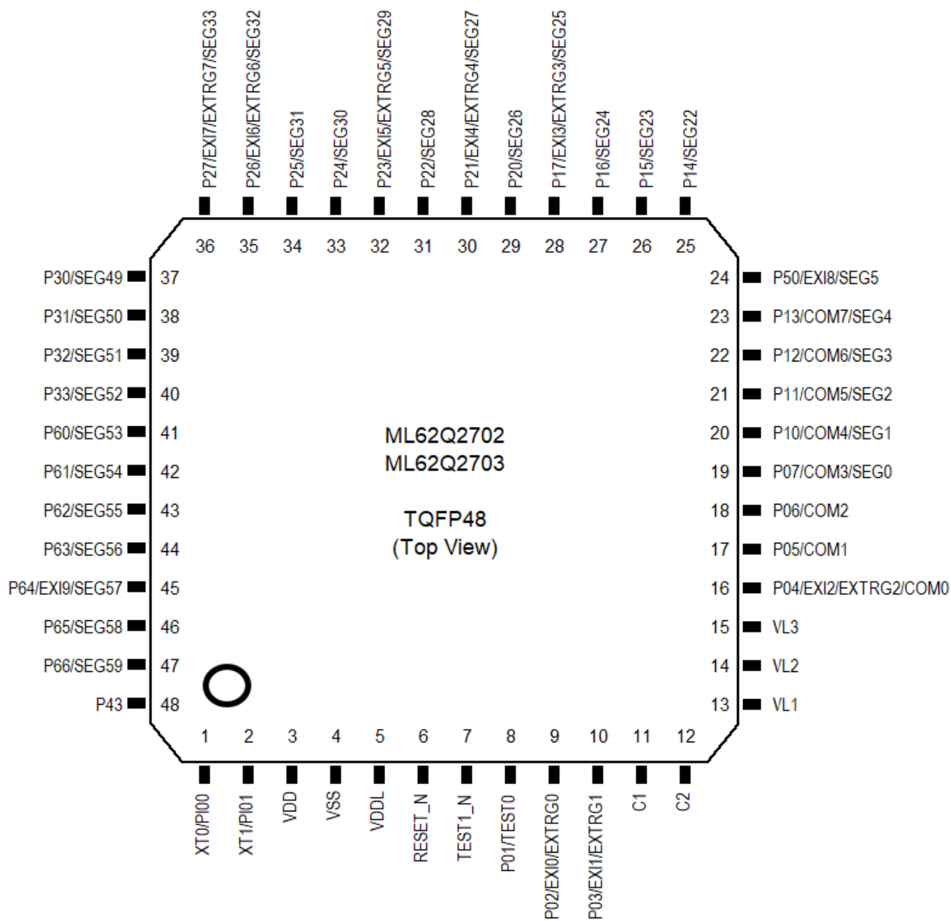
Fig.3-7 48 pin TQFP
