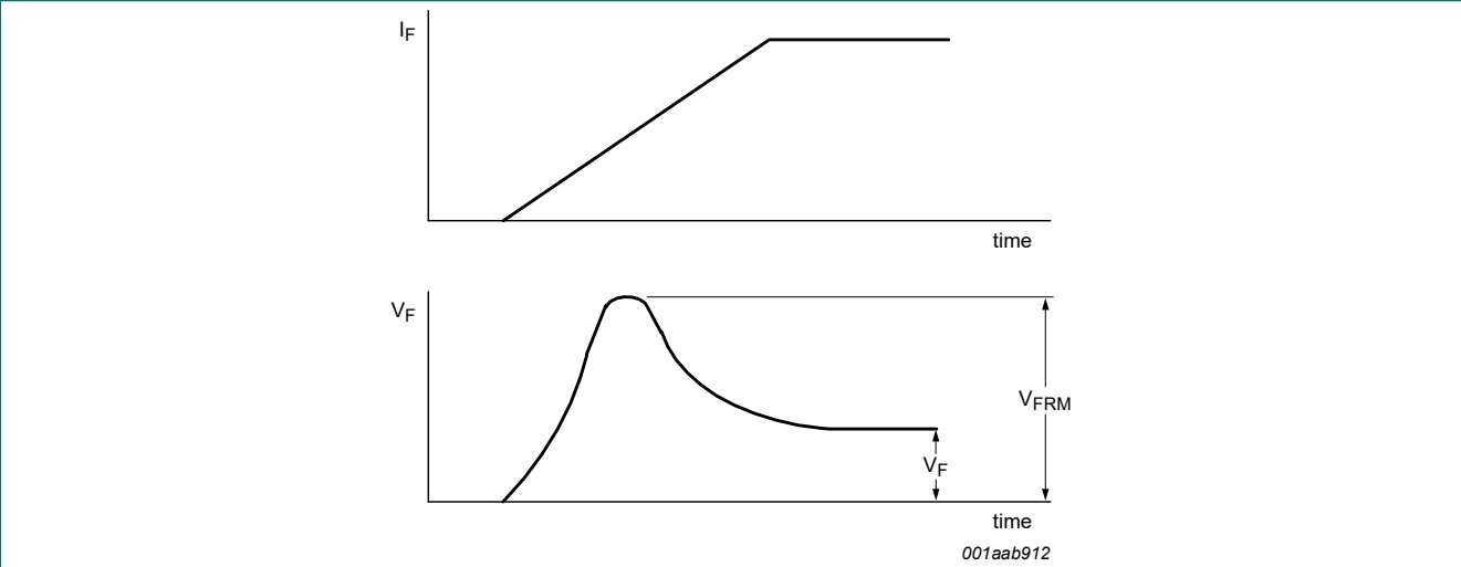
Fig. 10. Forward recovery definition
