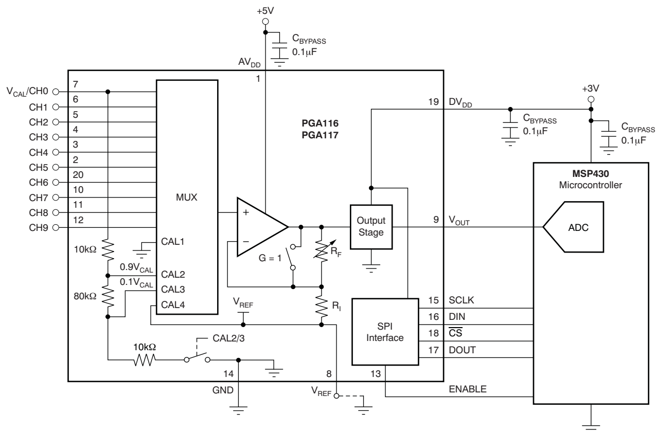
Figure 78. PGA116, PGA117 (TSSOP-20)
