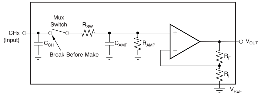
Figure 55. Equivalent Input Circuit
