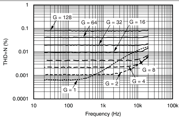
Figure 25. PGA112, PGA116 THD + NOISE vs Frequency ( V_{OUT} = 4\text{ V}_{PP} )
