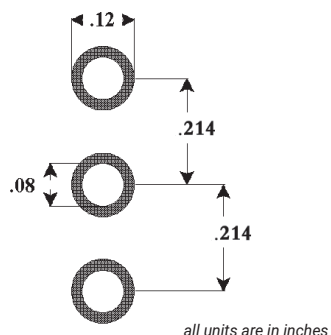
TO-247-3
