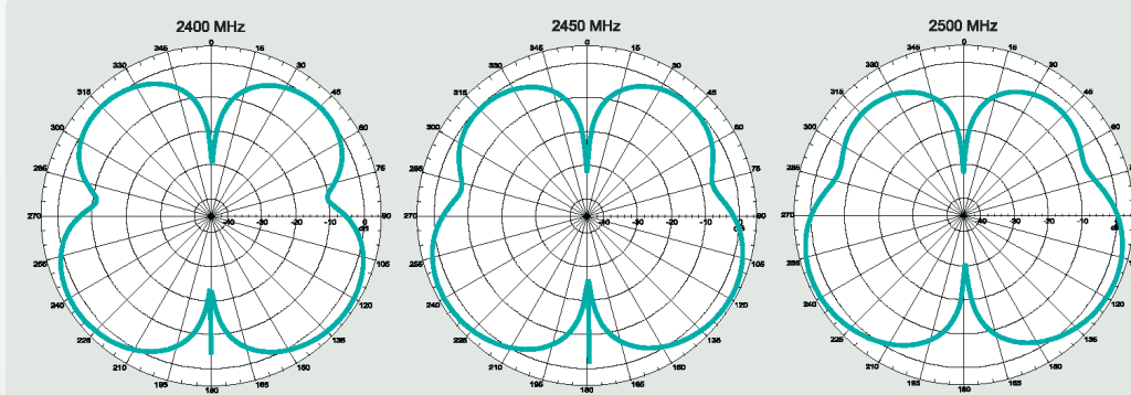
Figure 1.4: Pulse W1027 Antenna Gain Performance
