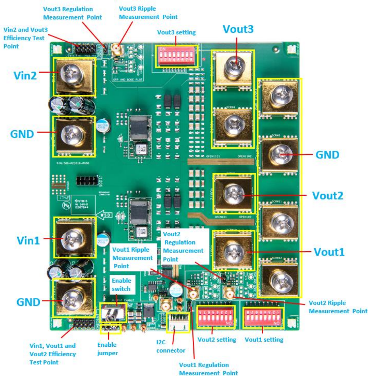
Fig. 2 – LGA50D setup
