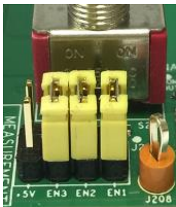
Fig. 9 – The enable jumpers – all 3 shown in place to enable all 3 outputs
