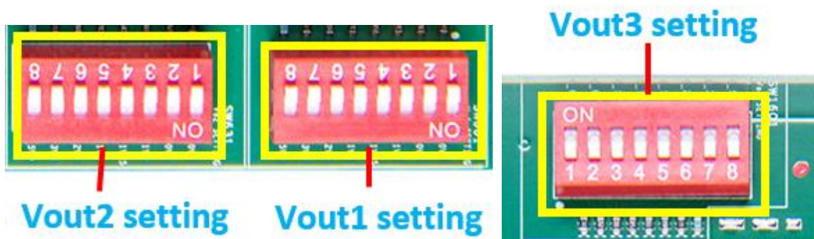
Fig. 6 – Nominal output voltage settings by DIP switch setting
