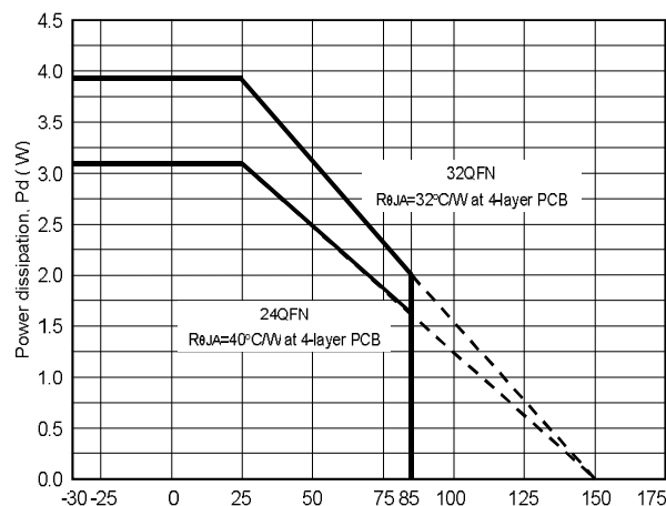
Figure 2. Maximum Power Dissipation
