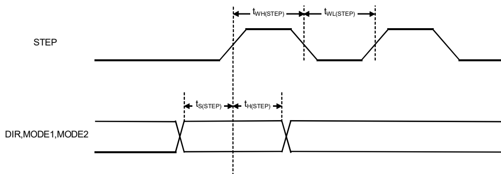
Figure 3. Timing Chart
