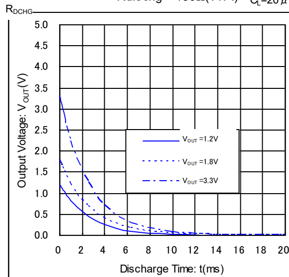
Output Voltage Discharge characteristics
