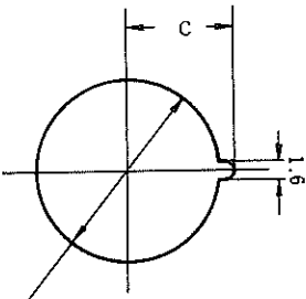
Mounting holes, for shell sizes 21, 24, 31
