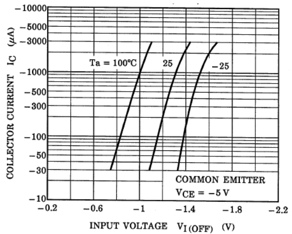
Fig. 14.4 Q2 I_C - V_{I(OFF)}
