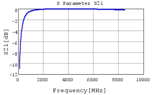
GCQ1555C1H4R7CB01 S21 DCOV, 25degC
