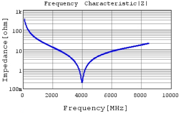
GCQ1555C1H4R7CB01 |Z| DC0V, 25degC
