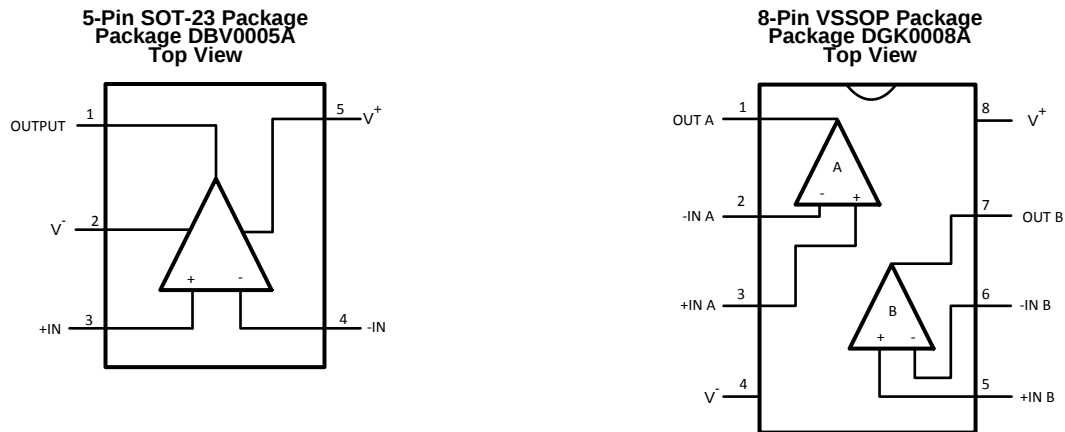
Pin Functions
