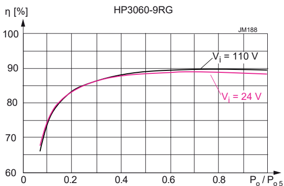
Fig. 7c Efficiency versus V_i and P_o (HP3060)
