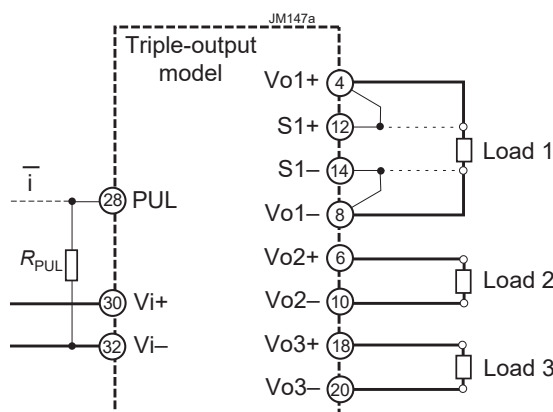
Fig. 1d Independent triple-output configuration. Output 3 is tracking
