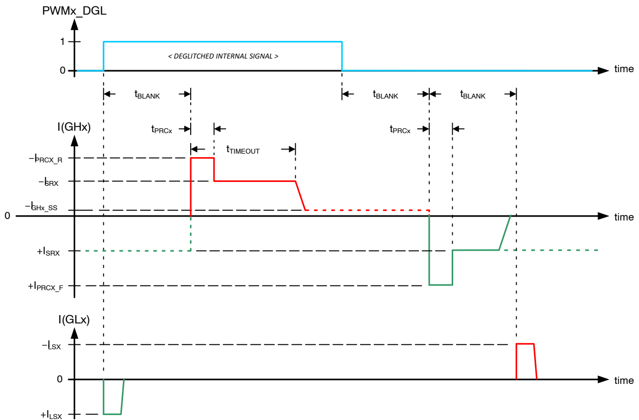
Figure 9. Gate Drive Current Evolution
