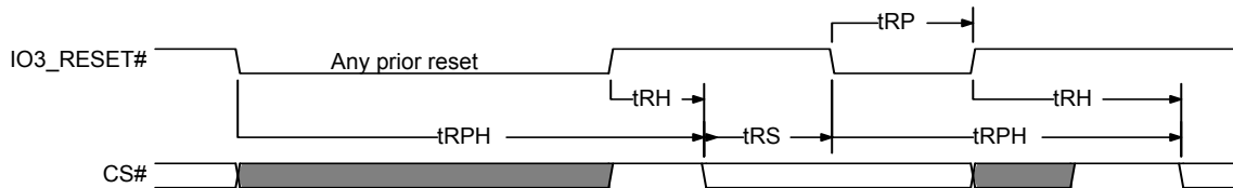
Figure 6.8 Hardware Reset when Quad or QPI Mode is not enabled and IO3_RESET# is Enabled
