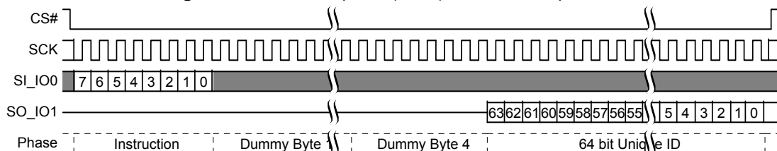
Figure 11.7 Read Unique ID (RUID) Command Sequence
