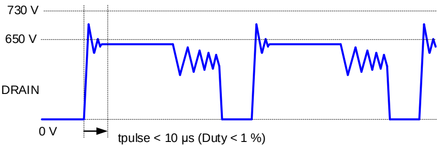
Figure 14. DRAIN pin Ringing Waveform
