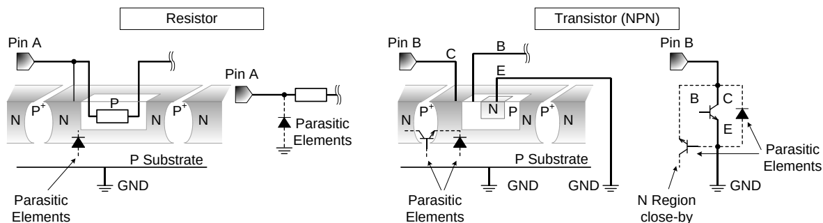
Figure 48. Example of IC Structure
