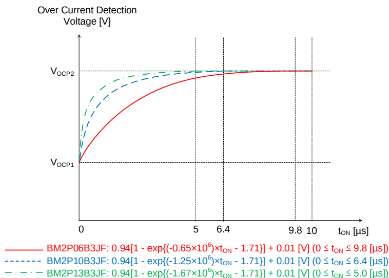
Figure 10. Over Current Detection Voltage
