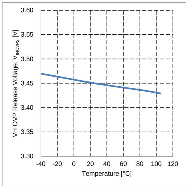
Figure 47. VH OVP Release Voltage vs Temperature
