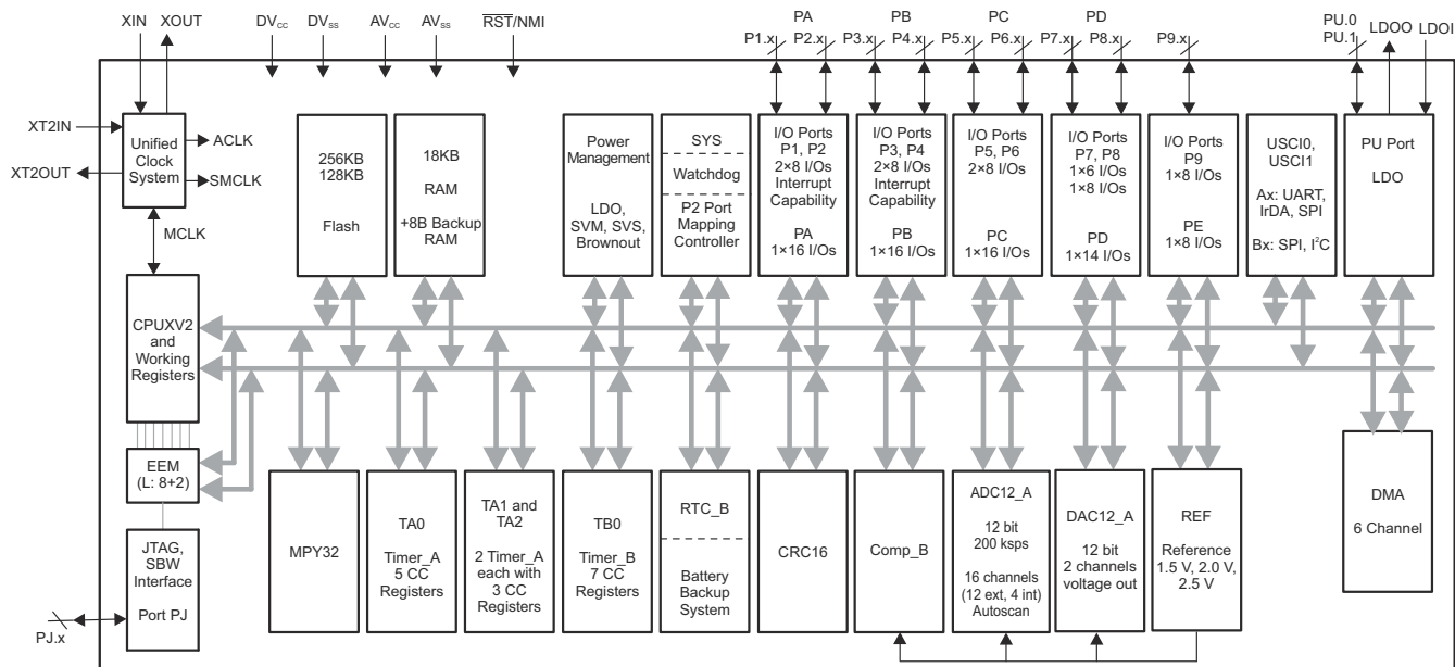
Figure 4-1. Functional Block Diagram – MSP430F5338, MSP430F5336
