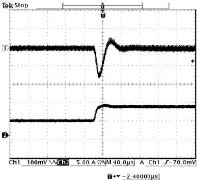
50% to 100% load 12 Vdc Input 1.2 Vdc Output
