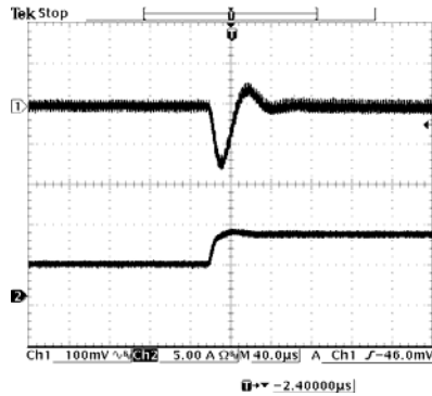
50% to 100% load 12 Vdc Input 0.9 Vdc Output
