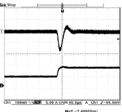
50% to 100% load 12 Vdc Input 1.8 Vdc Output
