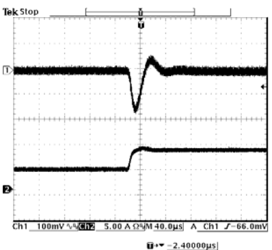
50% to 100% load 12 Vdc Input 1.5 Vdc Output
