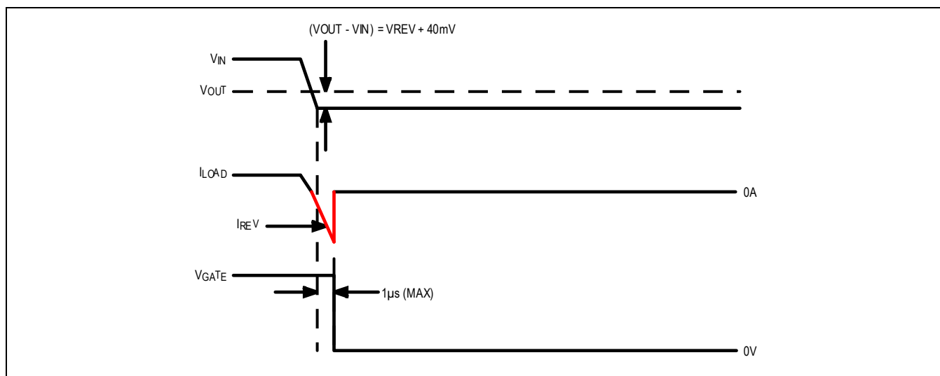
Figure 3. Reverse-Voltage Fault
