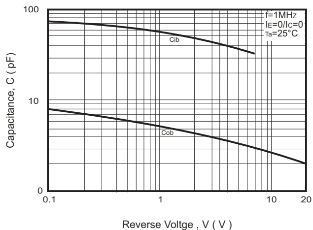
Fig. 7- C_{ob}/C_{ib} - V_{CB}/V_{EB}
