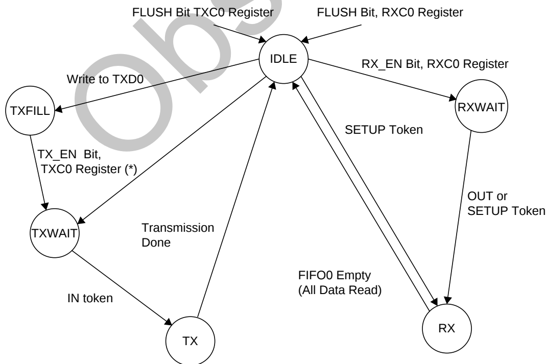
Figure 20. Endpoint 0 Operation
